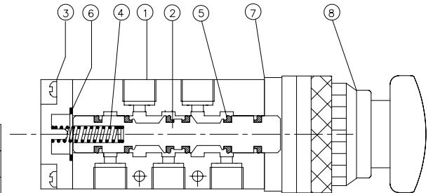
5/2 Mushroom button High Flow valve
