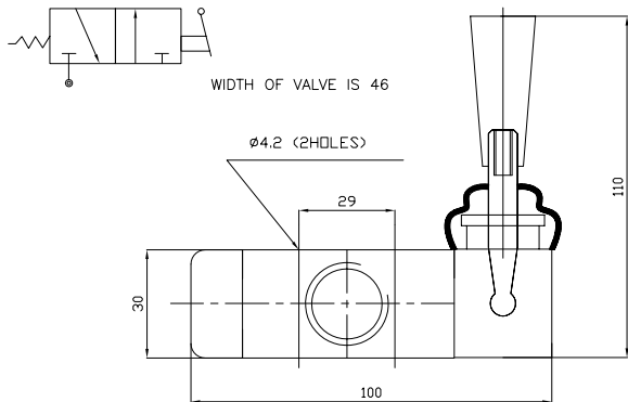
3/2 Hand lever High Flow Valve
