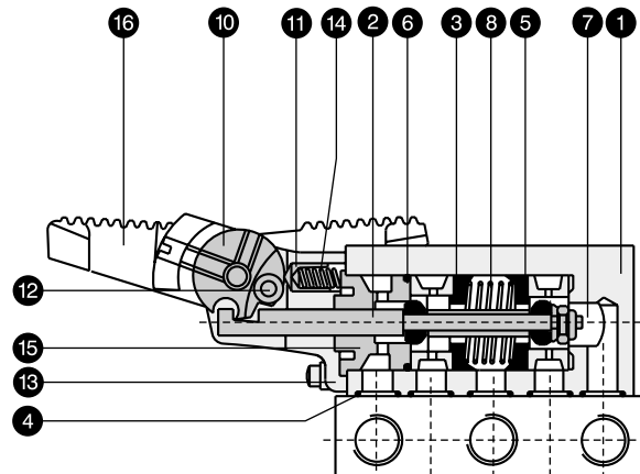
Foot Lever Operated Poppet Valve
