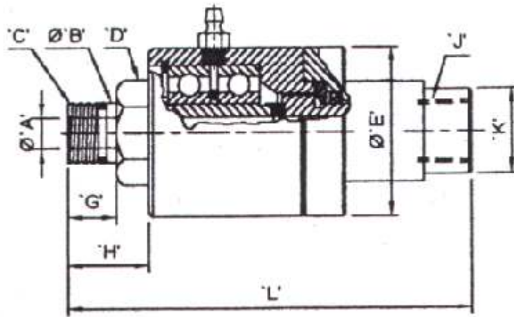
R-600 90° ROTARY UNION
